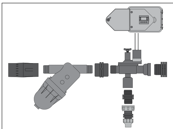
Connecting the main unit
