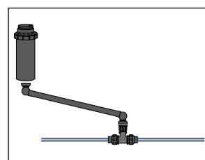
Connecting the pop-up sprinkler set
